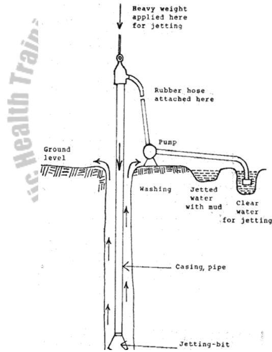
Fig.5.5. A jetted well
