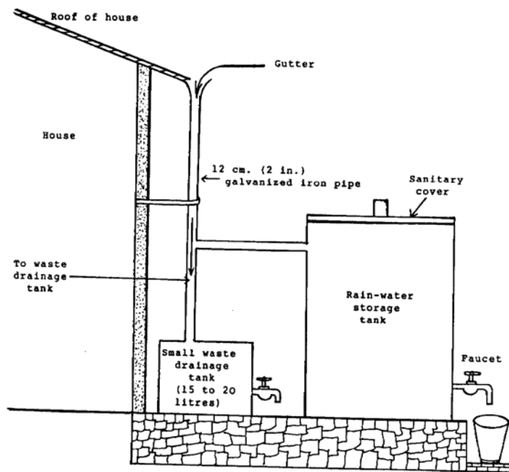
Fig. 5.10 A simple sanitary installation for collecting rainwater Source: Gebre Amanuel Teka, Water Supply in Ethiopia, 1973.
